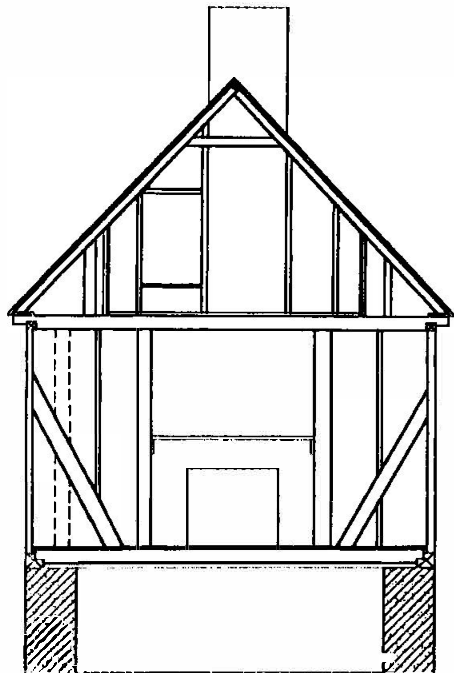
Framing Section B-B' View Looking West
