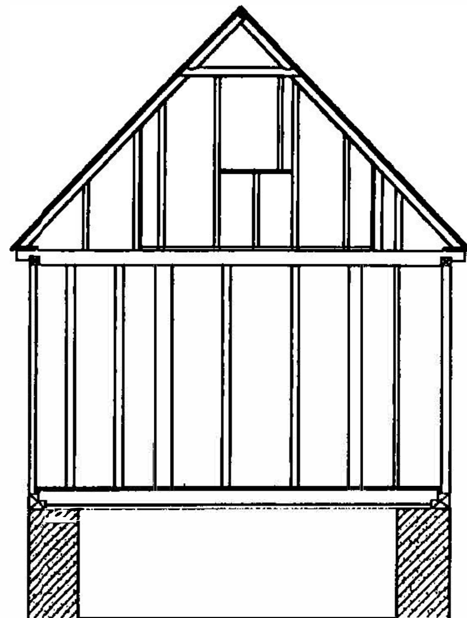
Framing Section C-C' View Looking East
